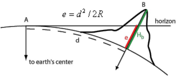
Figure 2: Earth's Curvature
