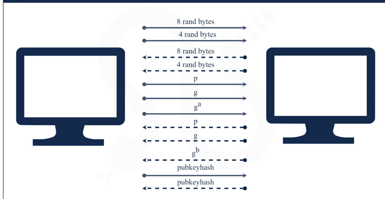
Figure 7: Snake Session Key Establishment
