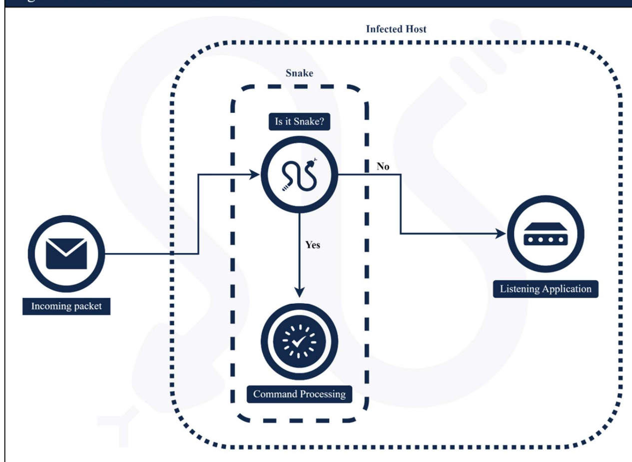
Figure 6: Snake Network Session Distinction
