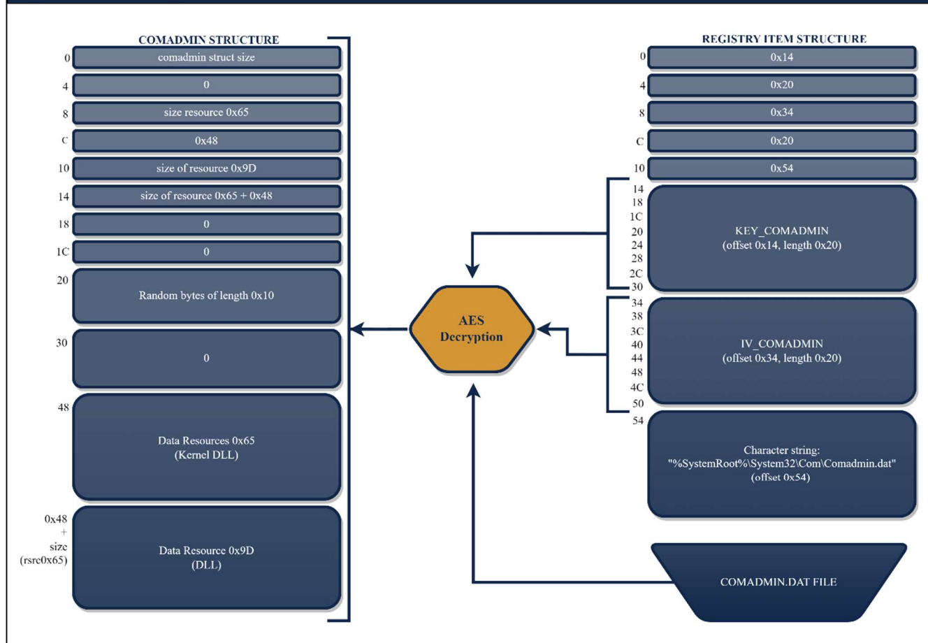
Figure 3: Driver Decryption Routine
