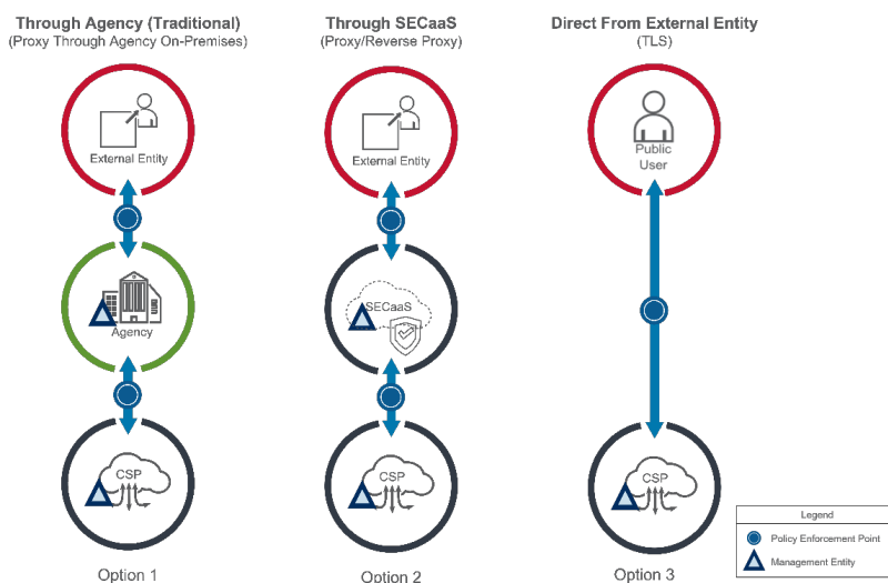
Figure 9: Security Pattern 3 – External Entity to Cloud Service Provider
