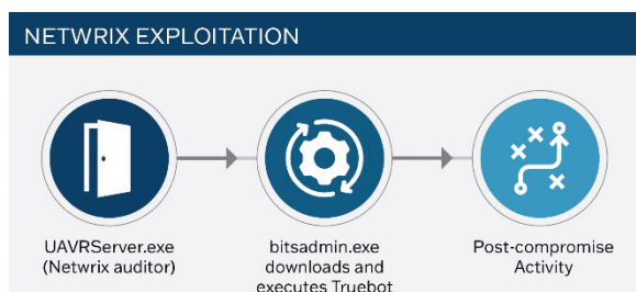
Figure 1: CVE-2022-3199 Delivery Method for Truebot
