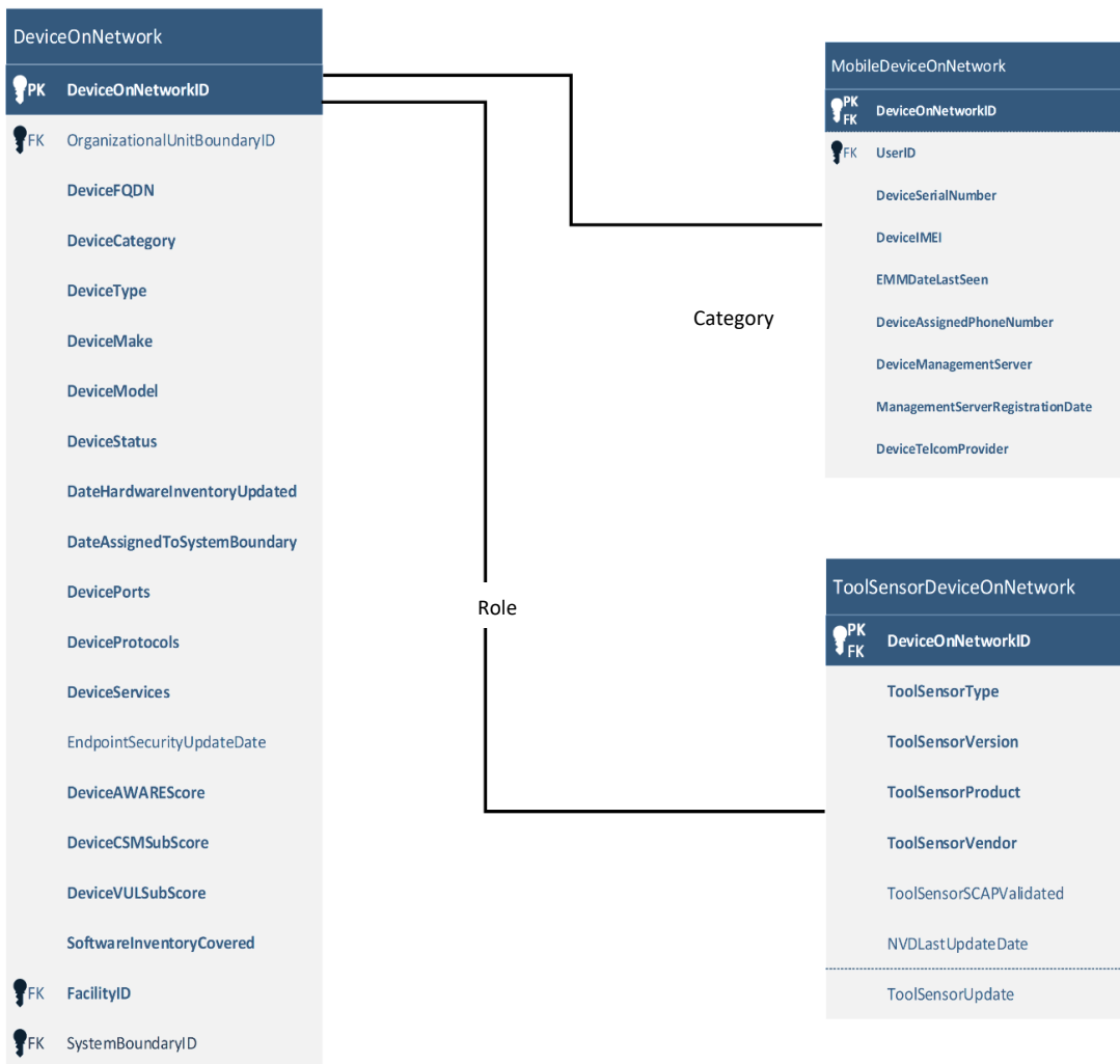
Figure 2-2: DeviceOnNetwork with Specializations
