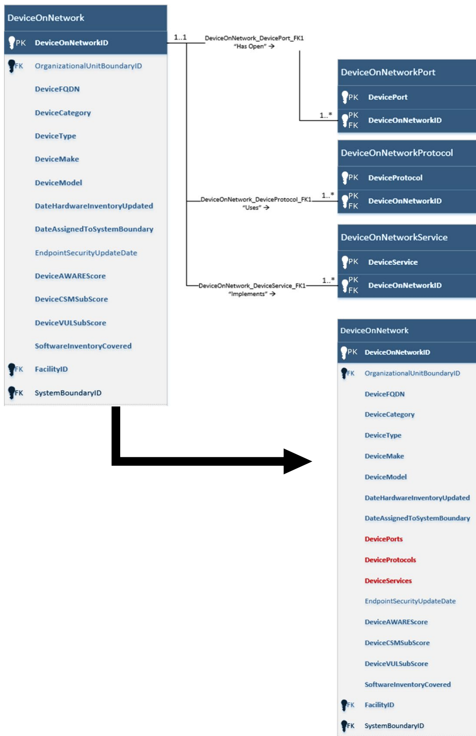
Figure 2-3: Multi-valued Attributes DevicePort, DeviceProtocol, and DeviceService
