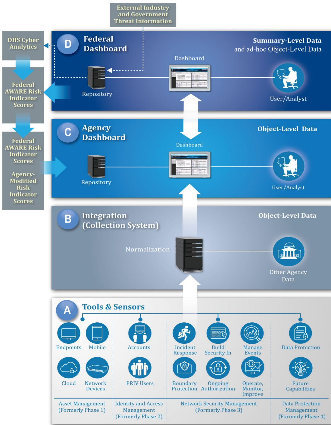
Figure 1-1: CDM "ABCD" Diagram
