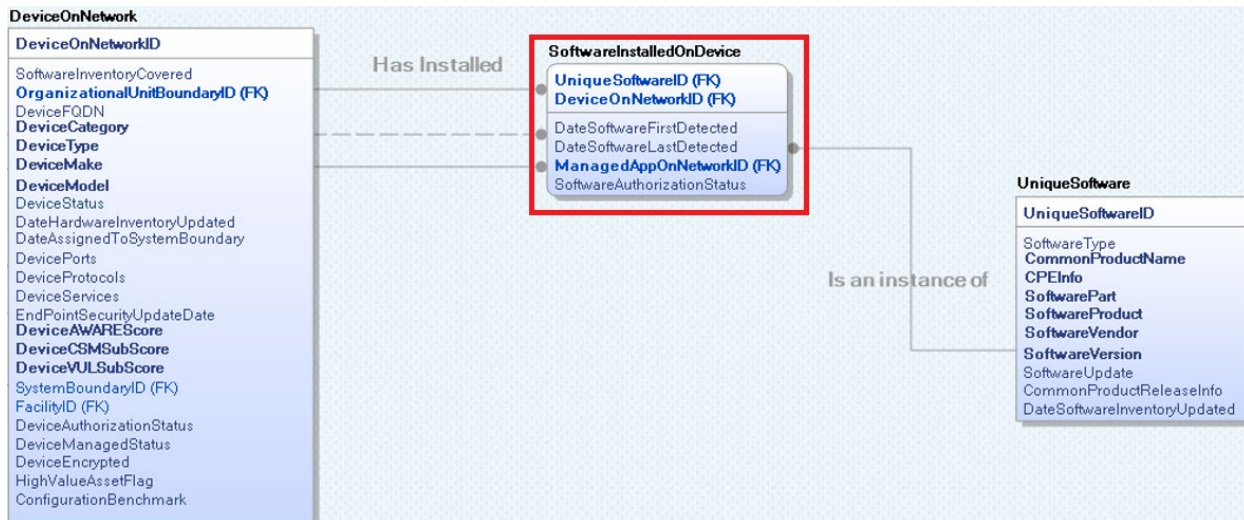
Figure 2-1: Relationship Between DeviceOnNetwork and UniqueSoftware
